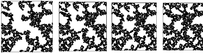
FIG. 5. Configuration of 1400-disk sample of series A without rolling resistance. Note the gradual closing of pores as the external pressure is increased from P^*=0 (first image) to P^*=0.01 (last image) going through two intermediate stages.
