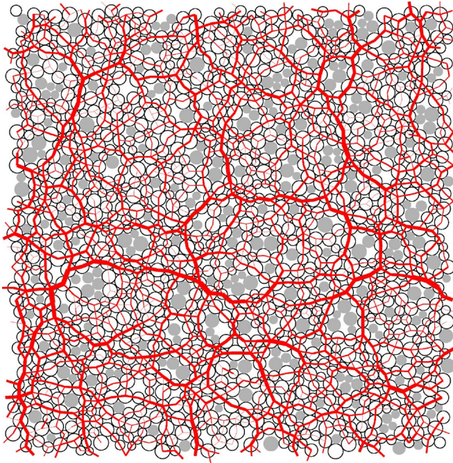
(a) No cohesion, K_N/P=10^5
