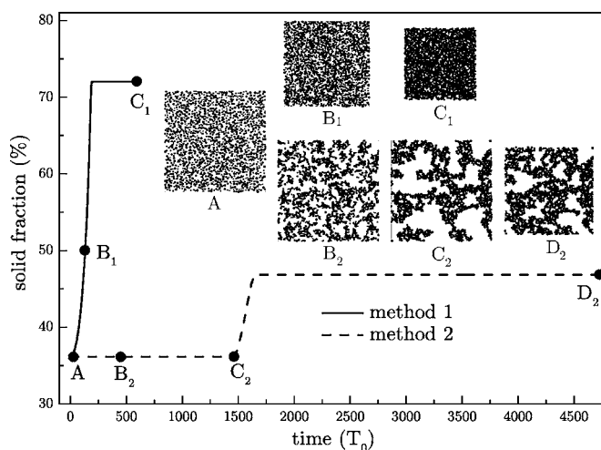
FIG. 4. Solid fraction versus time for both preparation procedures, showing some aspects of the configurations at different stages. Point A is the initial state (or \Phi_1 ). Aspects of configurations are shown for intermediate states B_1 and B_2 and for final equilibrated states C_1 and D_2 (at P^*=0.01 ). Point C_2 corresponds to the stage when all disks are assembled in a unique aggregate, then equilibrated at P^*=0 (both aggregation and equilibration stages take place between A and C_2 ). The time unit is T_0 = \sqrt{ma/F_0} . Note the duration of the preparation process with method 2 and the difference in final equilibrated states compared to method 1.
