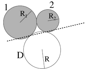
FIG. 16. The bottom disk, marked D, of radius R, is in contact with two other disks 1 and 2, themselves touching, whose radii are R_1 and R_2 . At equilibrium, contact forces on disk D should be carried by the dotted line joining its two contact points, which determines the ratio of tangential to normal force components.
