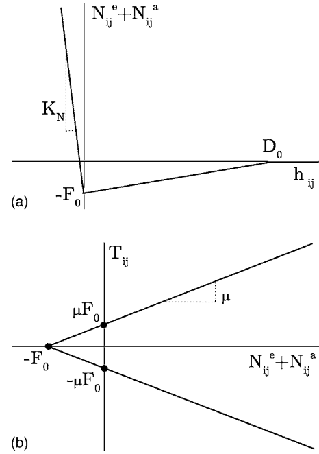
FIG. 1. Graphical representation of the model for the adhesive elastic contact force as a function of the distance between the surfaces of particles i and j , h_{ij} . (a) The elastic normal force consists of a repulsive Hookean part N_{ij}^e plus a linearized attractive part N_{ij}^a . (b) The elastic tangential force is limited by the Coulomb cone (adhesion shifting its tip to -F_0 on the normal force axis).
