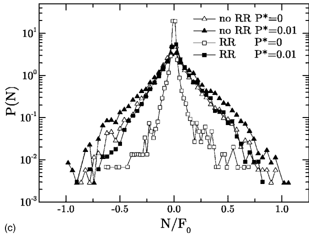
FIG. 9. Distribution of normal forces for series-A samples. The noncohesive case [(a)] is normalized by the average repulsive elastic part. The cohesive cases [(b) and (c)] are normalized by F_0 (note that the average of the elastic part of N is \langle N_e \rangle \approx F_0 in cohesive cases with P^* \ll 1 ).
