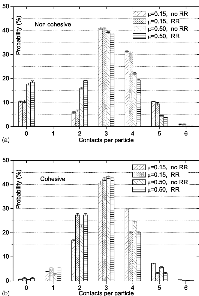
FIG. 3. Distribution of local coordination numbers (percentage of total particle number), without (a) and with (b) cohesion.
