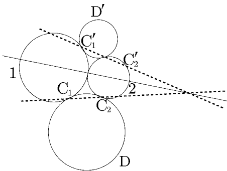
FIG. 18. Hyperstatic four-disk cluster, with five contacts. The force at the contact point between 1 and 2 should be carried by the continuous line joining this point to the intersection of the dotted lines. Those lines are respectively defined, as on Fig. 16, by the two contact points C_1 and C_2 of lower disk D with disks 1 and 2 and the two contact points C'_1 and C'_2 of upper disk D' with disks 1 and 2. Note that the solid line is close to the line of centers, hence a small value of ratio |T/N| in the contact between 1 and 2.
