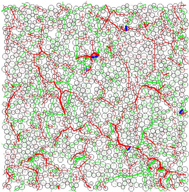
(b) Cohesive system, \kappa=10^5 , P^*=0.01
