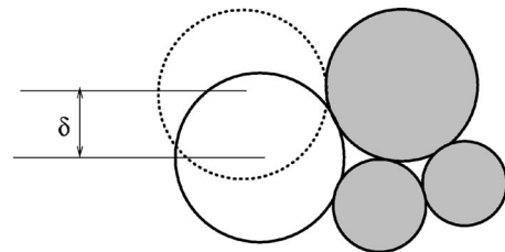
FIG. 13. Three (gray) disks initially forming an isostatic structure; when a fourth one (coming from the left) adheres to one of them (dotted position), it can roll (this is a floppy mode) until another (fifth) contact is formed, stabilizing it in the final position drawn with a solid line. The final “double-triangle” structure is hyperstatic. Final forces (see main text) were computed for different initial velocities of the mobile disk and for different values of impact parameter \delta .
