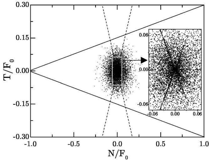
FIG. 17. Values of normal and tangential contact forces in a 5600-disk, type-2 sample of monodisperse disks in equilibrium under P^*=0 . Note the sharp “X” shape on the blown-up detail of small forces.
