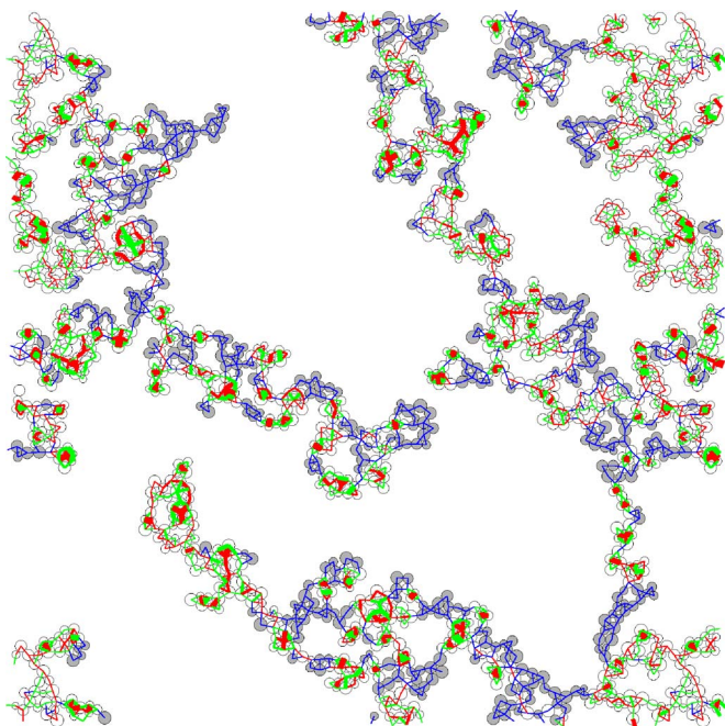
FIG. 11. (Color online) Sample of type 2 ( N=1400 ), in equilibrium under P^*=0 after aggregation stage, with solid fraction \Phi=0.26 (series B ). Same conventions as on Fig. 2, except for the blue color corresponding to contacts carrying a total force below tolerance 10^{-4}F_0 (deflection h_0 and no mobilization of tangential force). Note the large number of such interactions and the local compensation of attractions and repulsions in small prestressed clusters. To help visualize unstressed regions, disks only interacting at contacts bearing forces below tolerance are filled in light gray.
